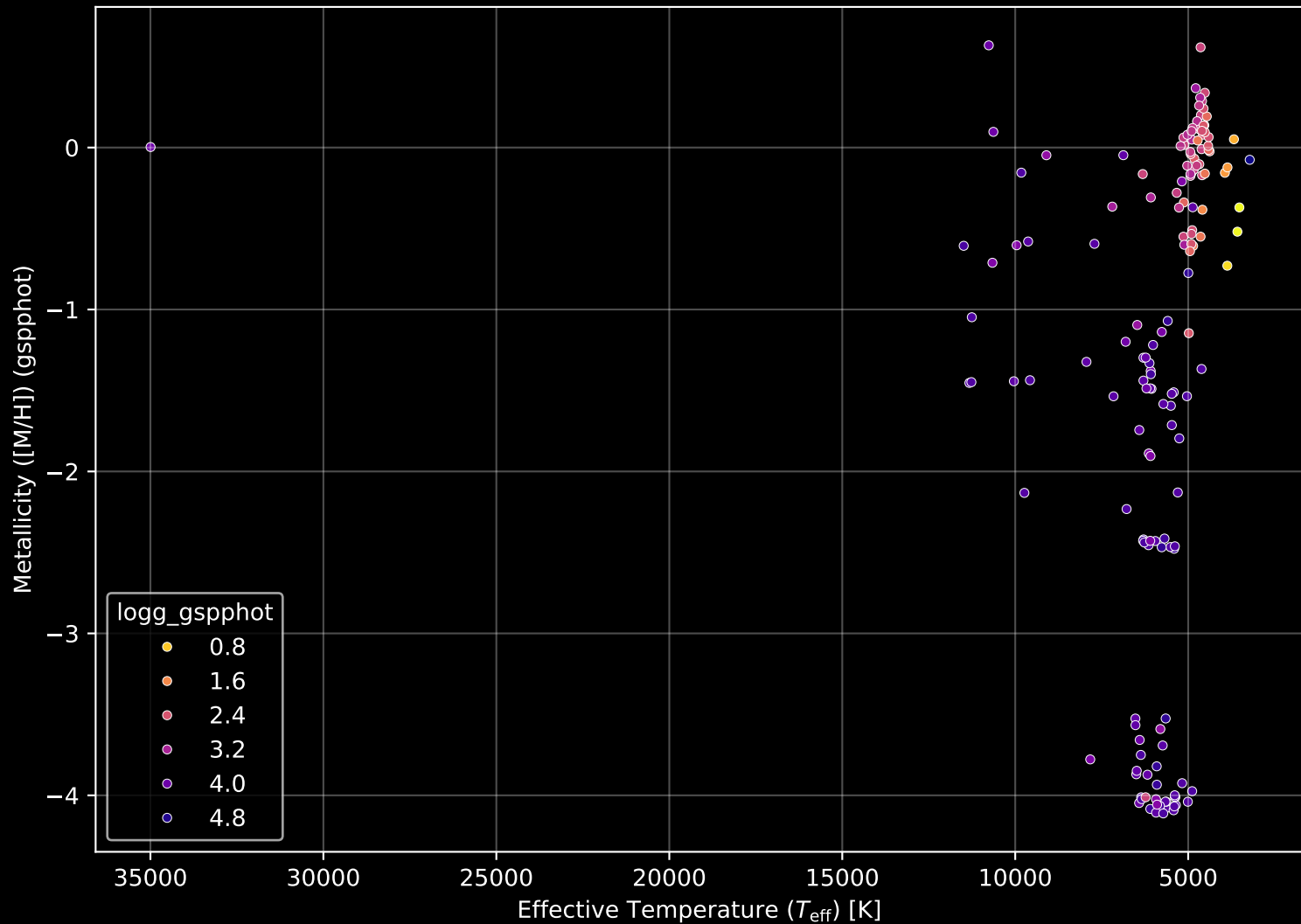
APOGEE DR17 Field: [358-05-O] Stellar Population Parameters (n= 161)
