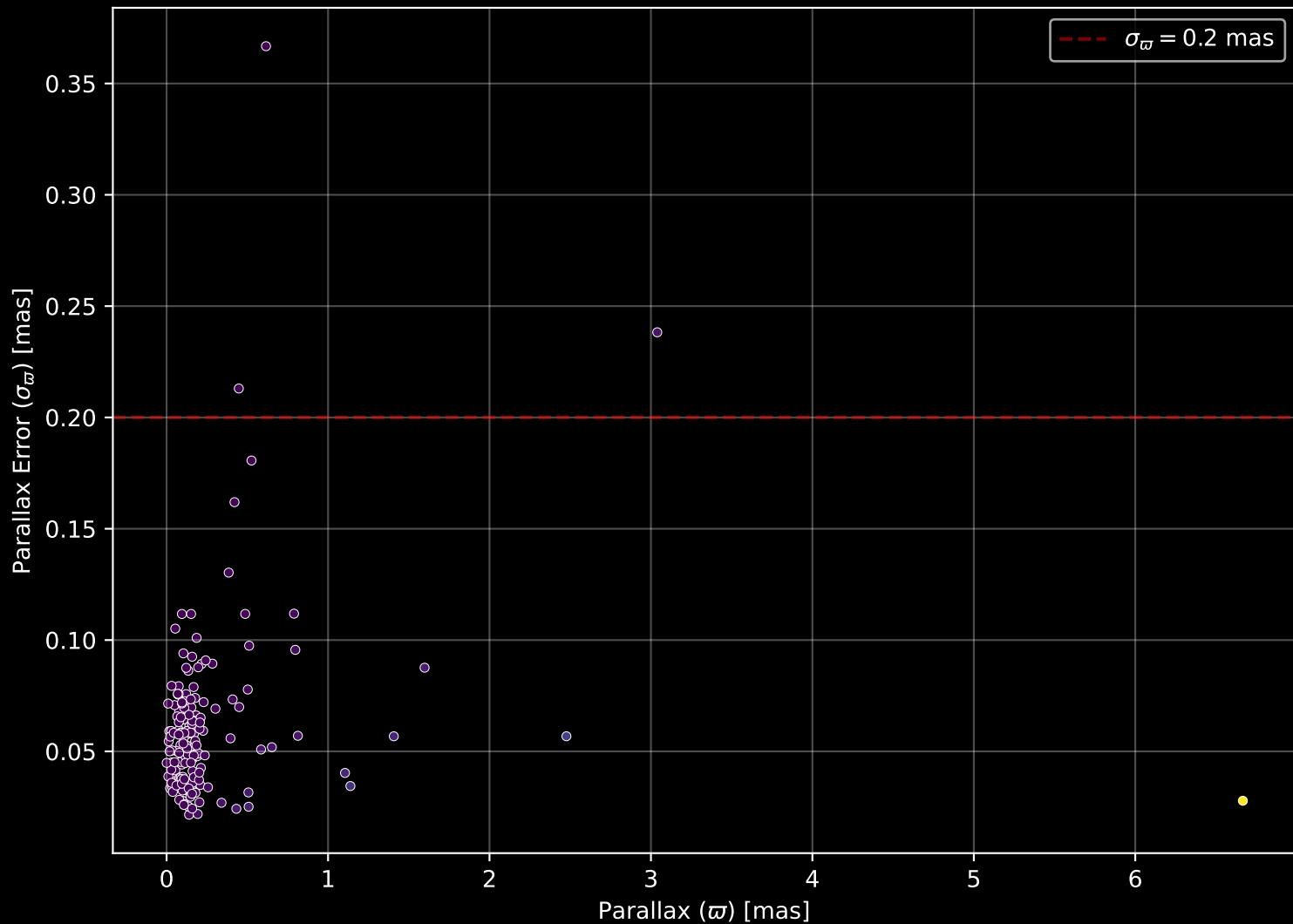
APOGEE DR17 Field: [358-05-O] Parallax Quality (n= 161)
