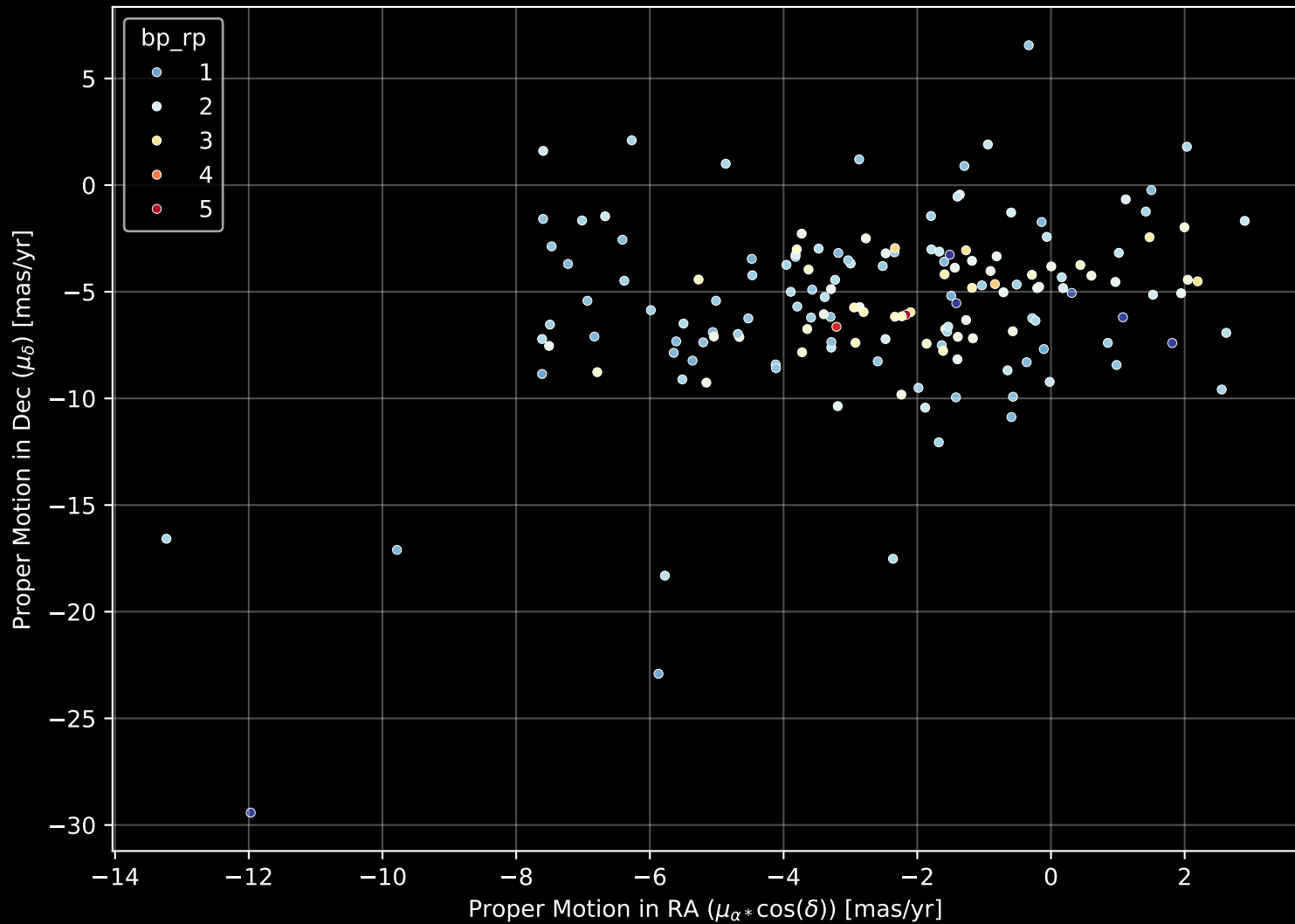
APOGEE DR17 Field: [358-05-O] Proper Motion Diagram (n= 161)
