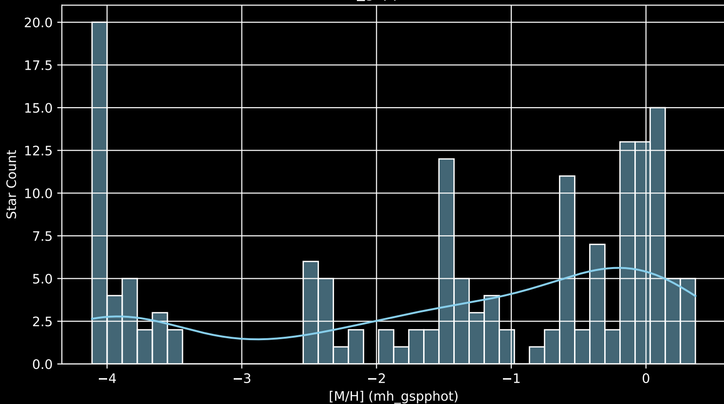
APOGEE DR17 Field: [358-05-O [M/H] (mh_gspphot) (n= 159)
