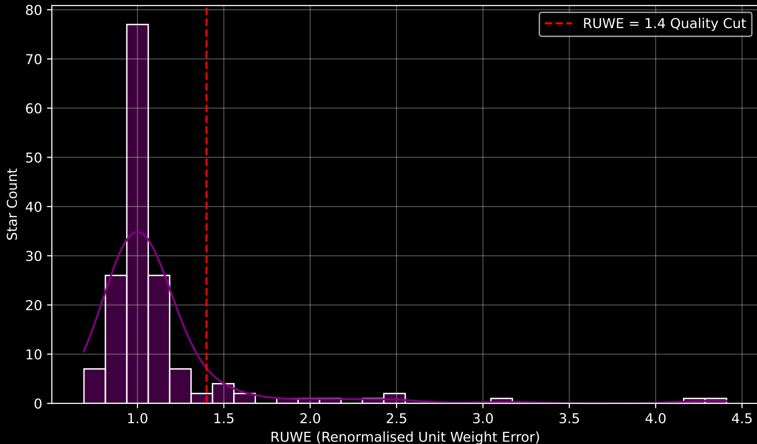
GAPOGEE DR17 Field [358-05-O] RUWE Distribution (n= 160)
